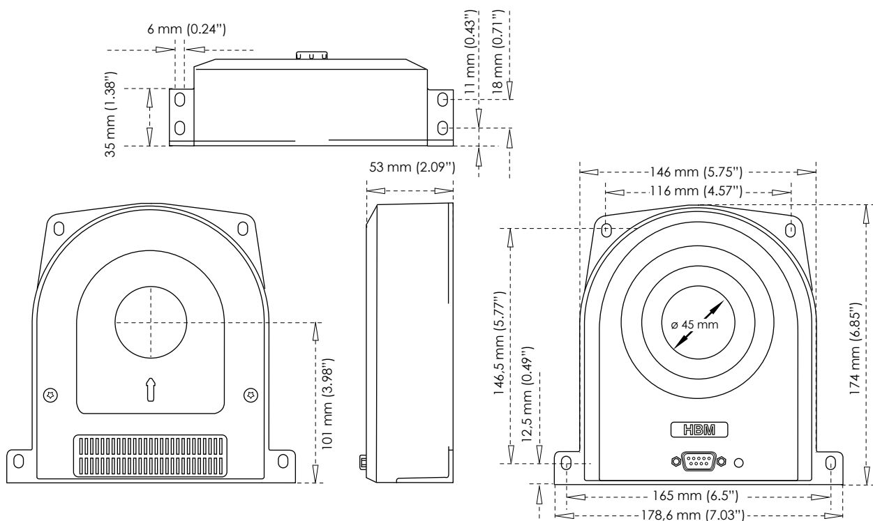
Figura 1.5: Dimensioni CTM1200ID/CTM1200ID-CD3000
