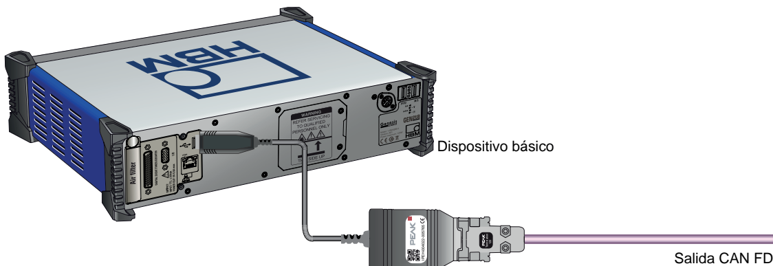
Figura 31: Salida CAN FD autónoma GEN2tB
