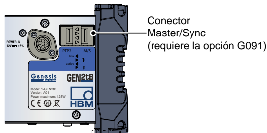
Figura 12: Conector Master/Synch
