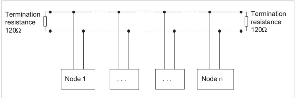
Fig. 9.1 Bus termination resistors
