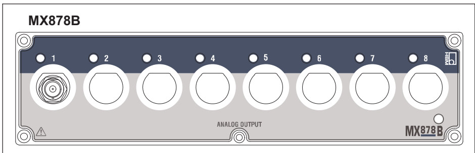
Fig. 10.2 MX878B front view
