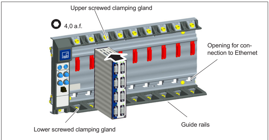
Fig. 6.17 Mounting the module
