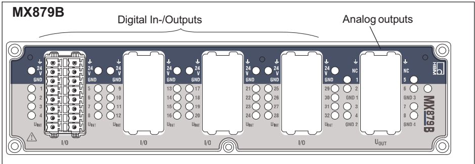
Fig. 10.3 MX879B front view
