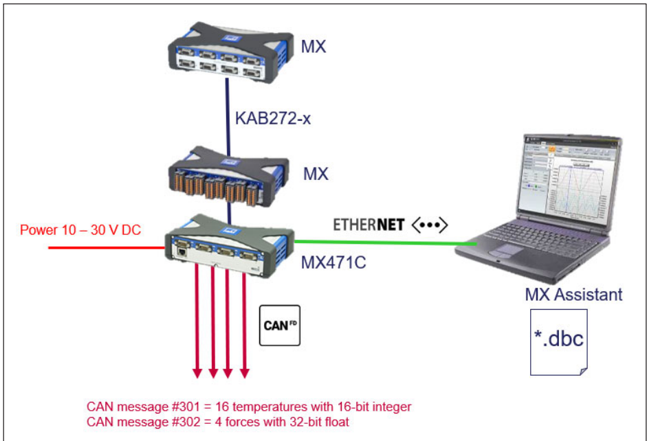
Fig. 7.9 Output to CAN bus (MX471C, every connection)
