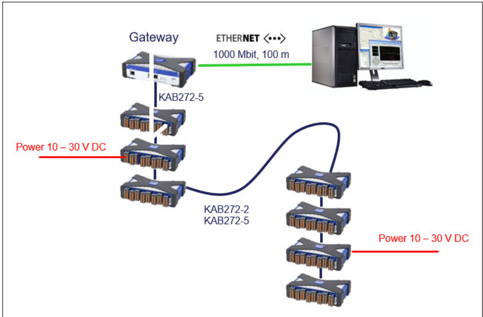
Fig. 7.6 Example of distributed setup
