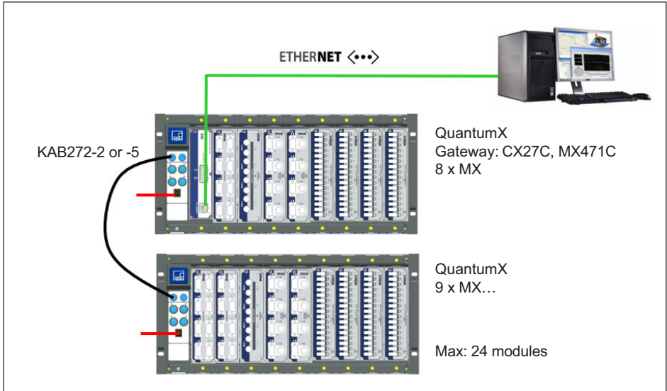
Fig. 6.21 Synchronizing multiple backplanes
