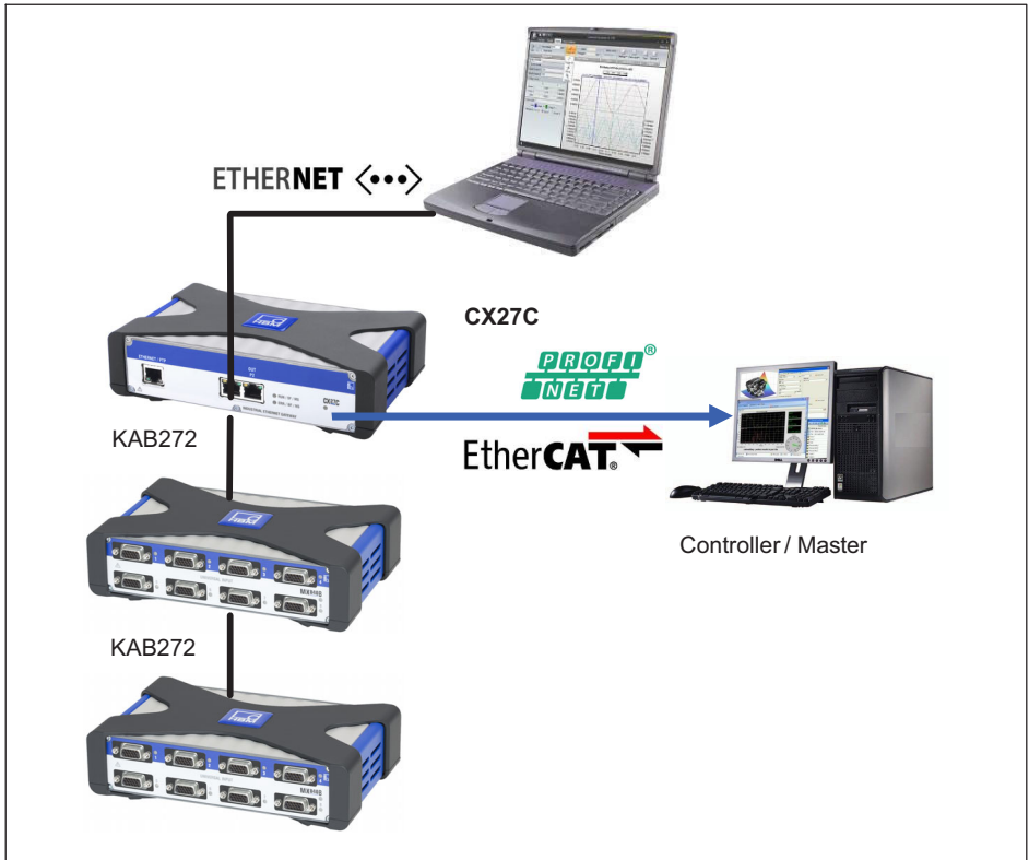
Fig. 7.11 Output in real time via the fieldbus and in parallel via Ethernet
