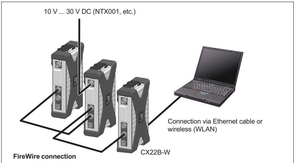
Fig. 7.7 Layout with CX22-W
