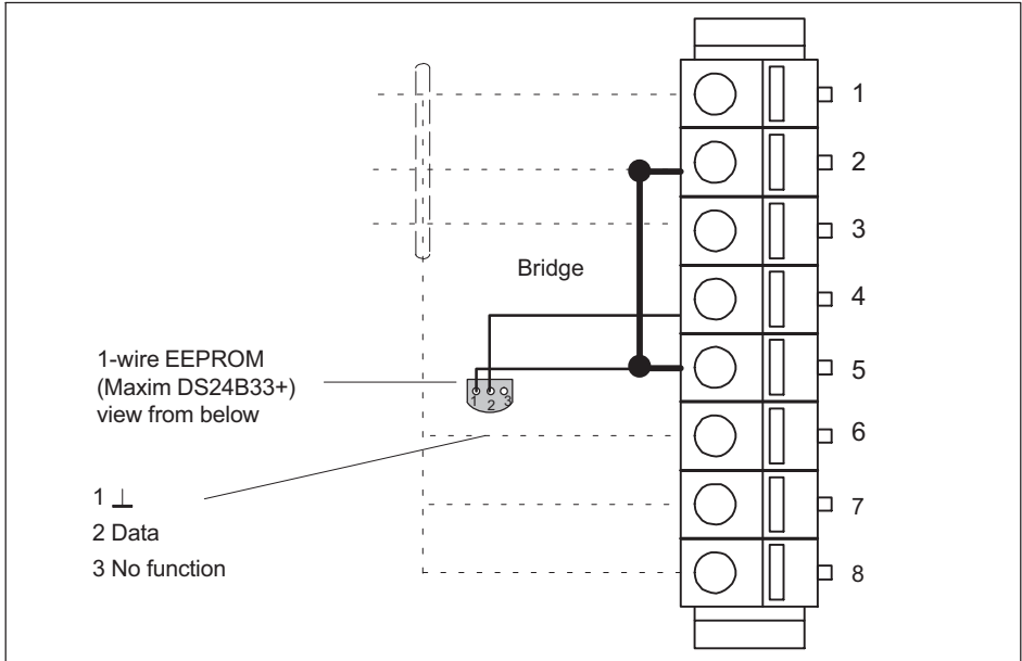
Fig. 8.16 Pin arrangement of connection plug, view from the connection side
