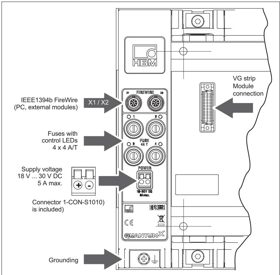
Fig. 6.12 BPX001 connections
