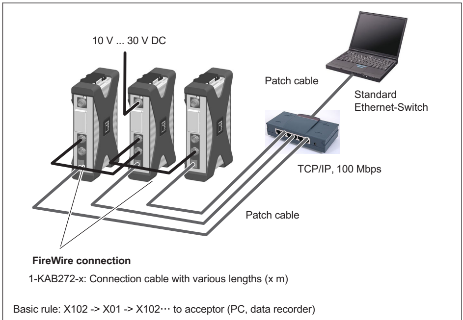
Fig. 7.4 Example of multiple connection via Ethernet with FireWire synchronization
