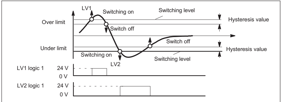
Fig. 10.4 Limit value functions and parameters
