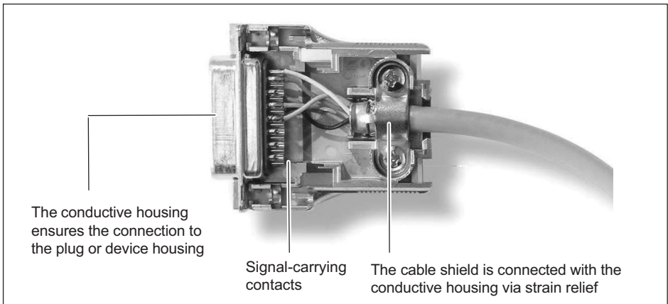
Fig. 8.1 Routing of the cable shield on the plug
