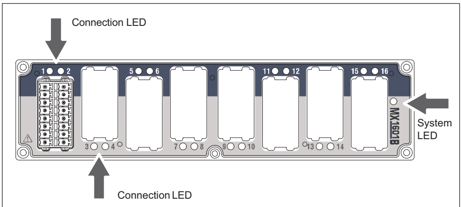
Fig. 8.17 MX1601B front view
