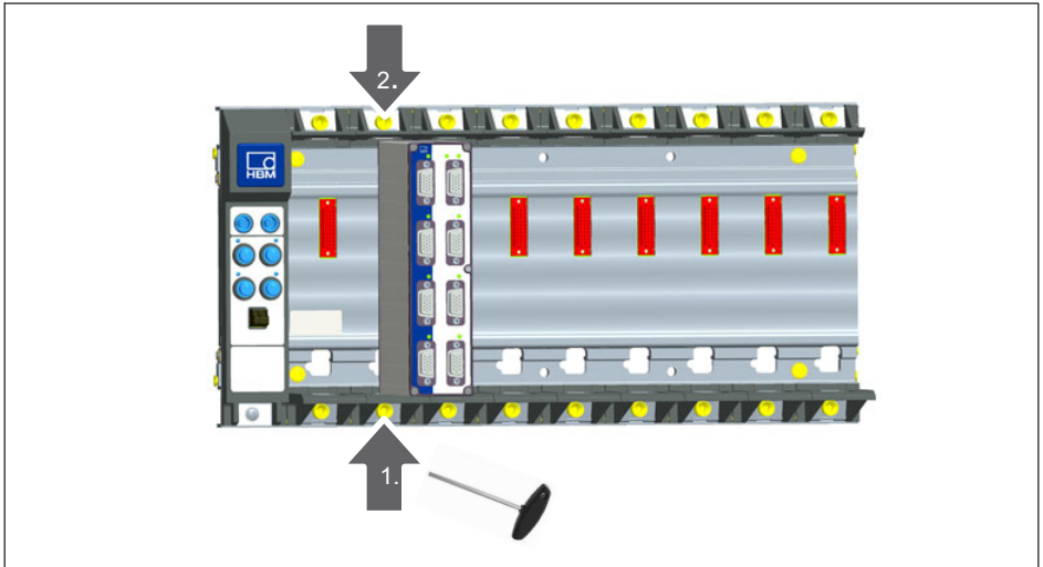
Fig. 6.19 Tightening the screwed clamping glands, sequence
