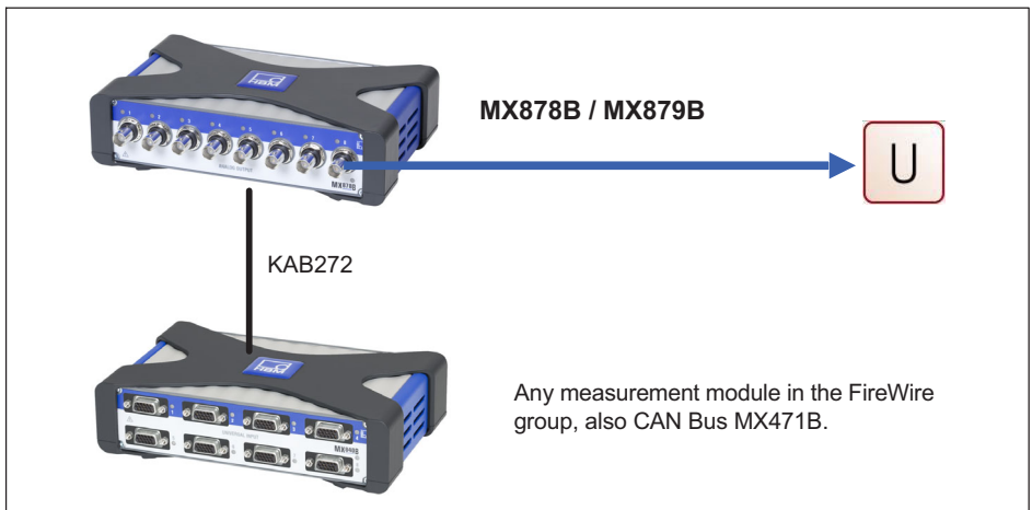
Fig. 7.10 Analog output in real time
