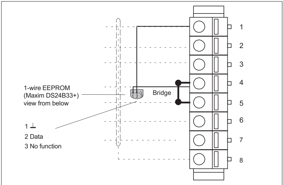
Fig. 8.18 Pin arrangement of connection plug, view from the connection side
